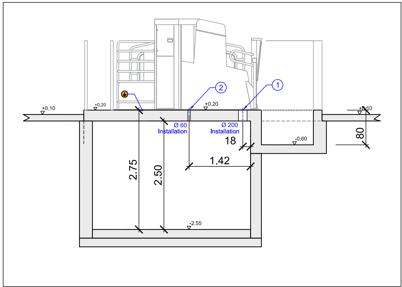
Sectional View - Installation
