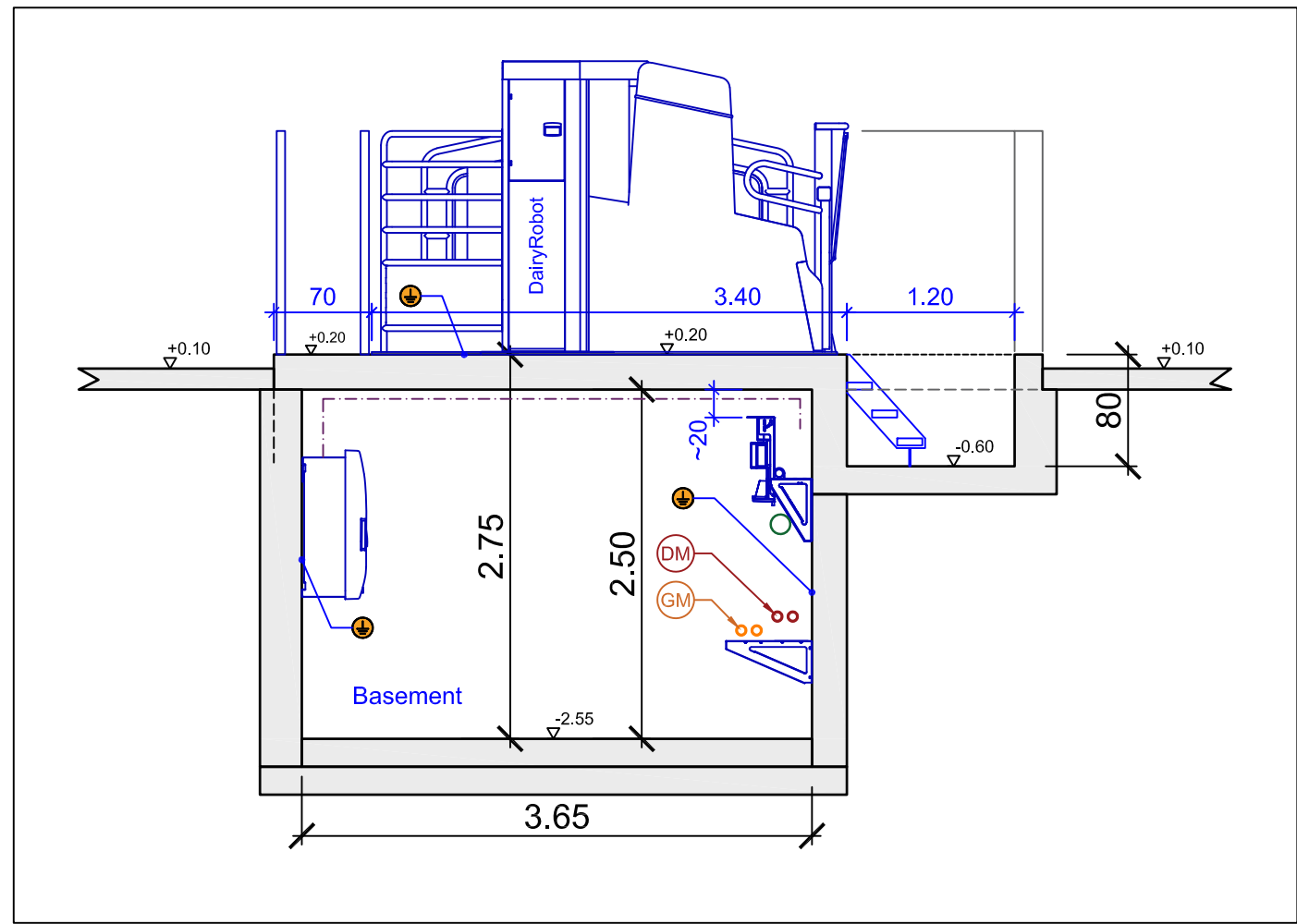
Sectional View - Equipment
