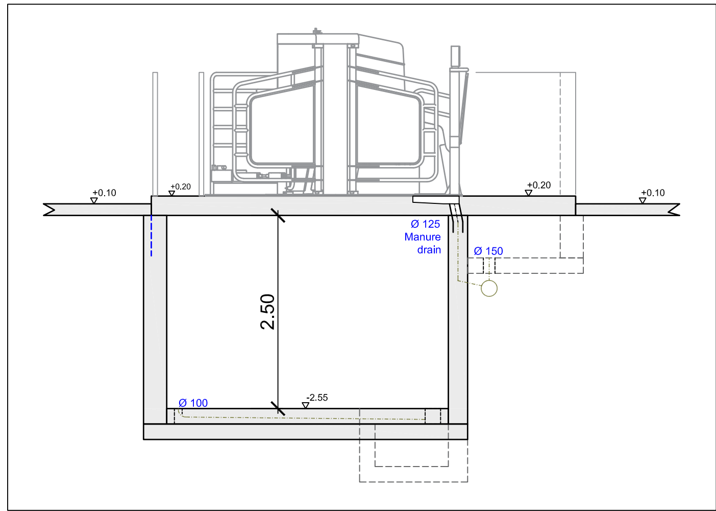
Sectional View - Drainage
